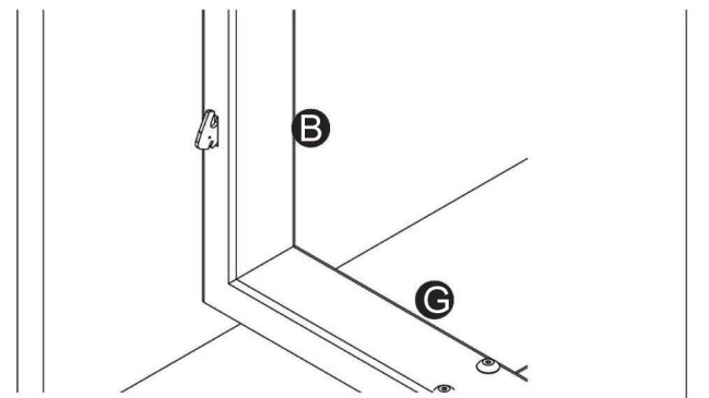
6 Insertion of basket hook
